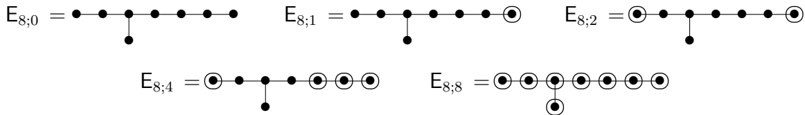
Figure 1: The opposition diagrams of type E_8
