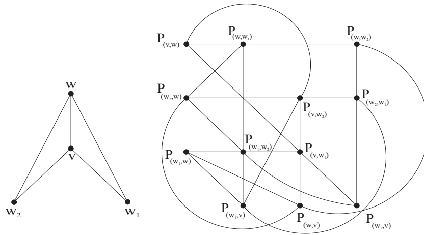
Figure 3: \mathcal{G}(V, E) does contain triangles
