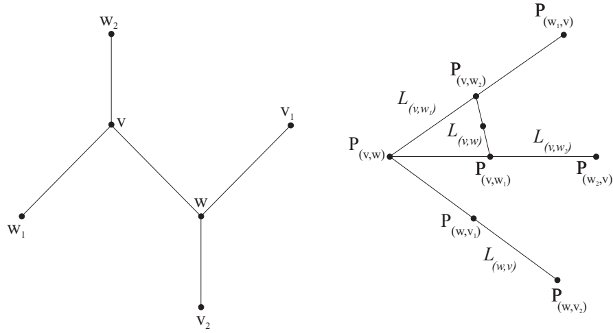
Figure 2: \mathcal{G}(V, E) does not contain triangles
