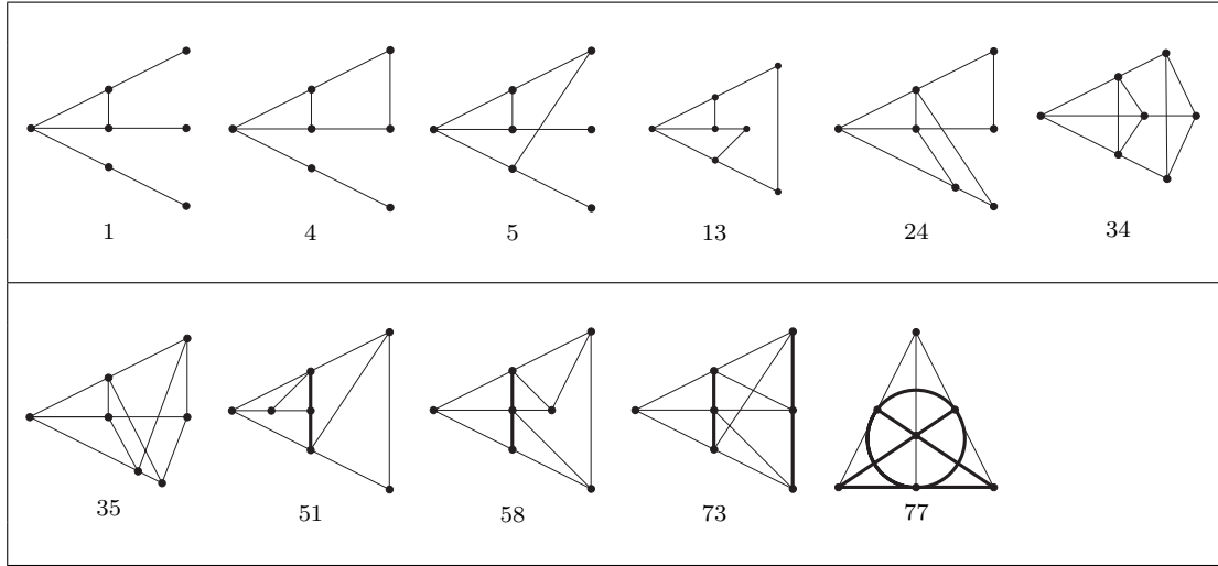
Figure 1: Local structure in a geometrically point homogeneous bislim geometry of gonality 3
