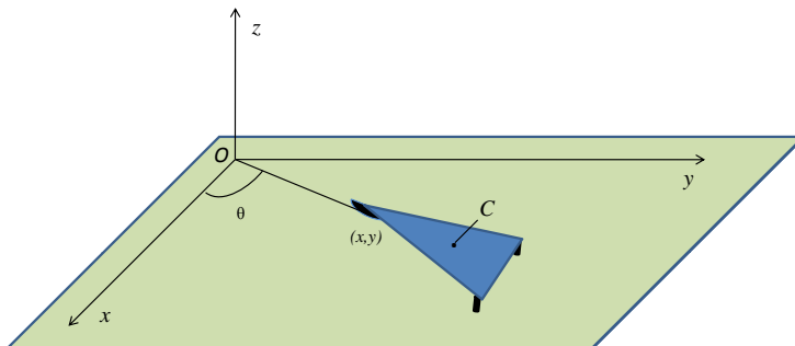
Figure 3: The Chaplygin Sleigh.
